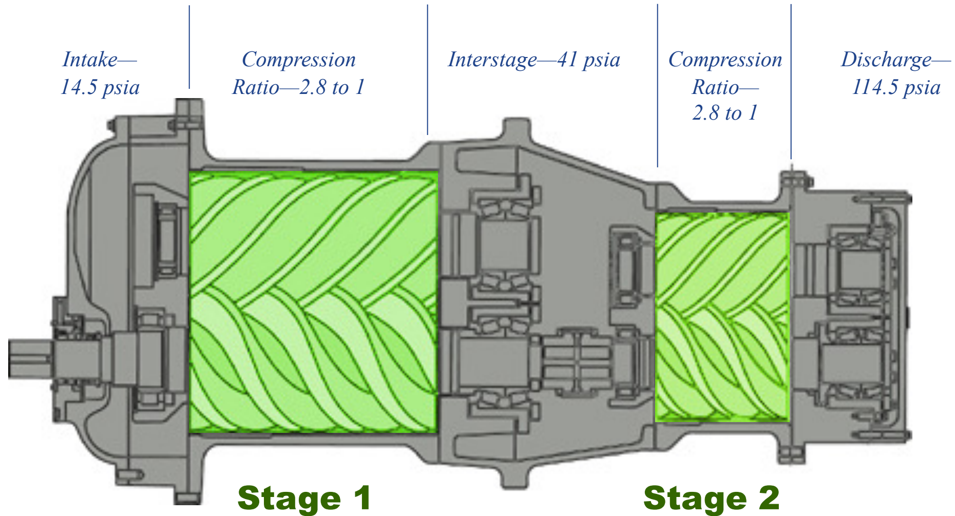
Two-stage Compressor
